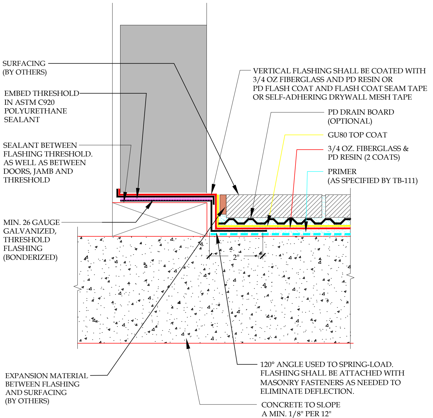
DETAIL-CON-DEK "U" SYSTEM - DOOR PAN FLASHING SCALE: N.T.S.
