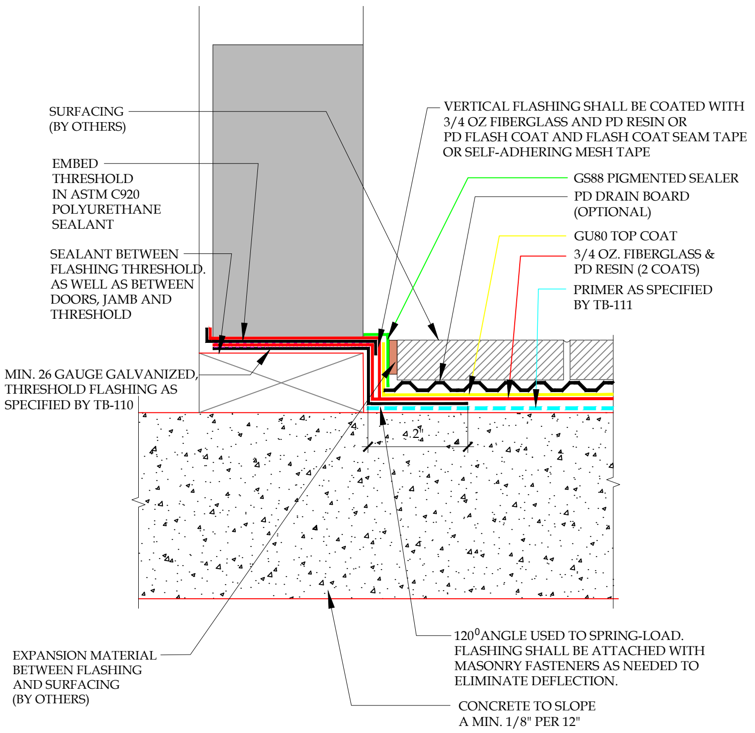
DETAIL-CON-DEK "U" SYSTEM - DOOR PAN FLASHING - INCLEMENT WEATHER SCALE: N.T.S.
